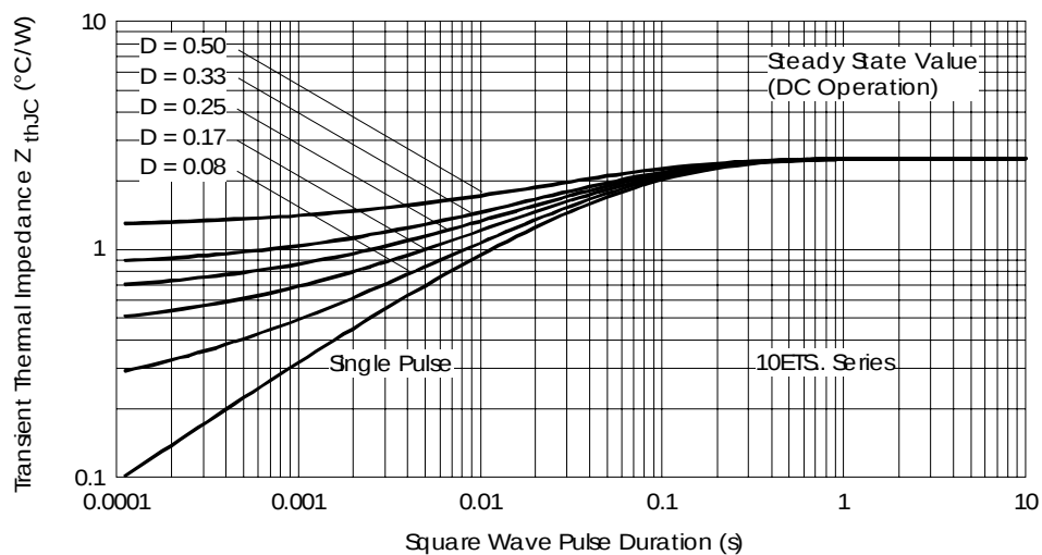
Fig. 9 - Thermal Impedance Z_{thJC} Characteristics
