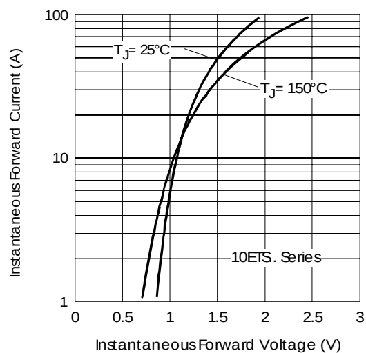
Fig. 8 - Forward Voltage Drop Characteristics
