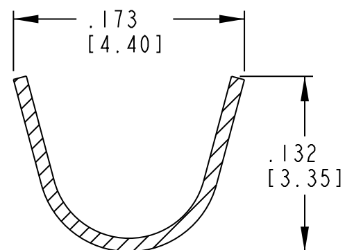
SECTION B-B INSULATION WINGS
