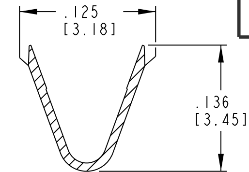
SECTION A-A CONDUCTOR WINGS
