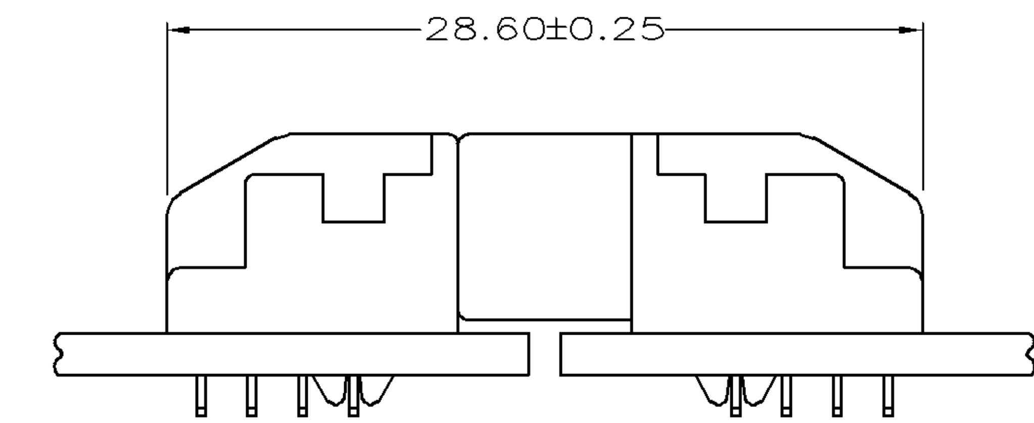
RIGHT ANGLE PLUG ASSEMBLY MATED TO RIGHT ANGLE RECEPTACLE ASSEMBLY
