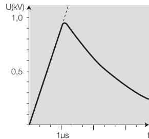
Pulse form shape without GDT
