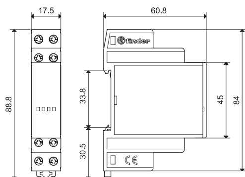
13.61 Screw terminal
