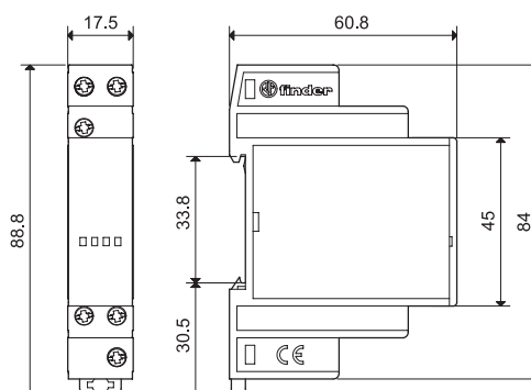
13.31/13.91 Screw terminal
