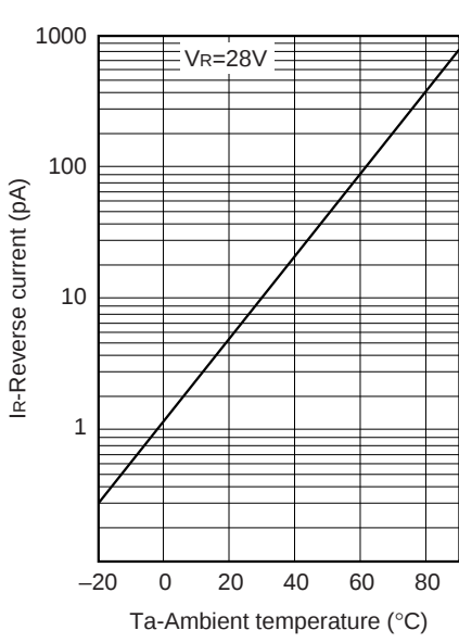
Reverse current vs. Ambient temperature
