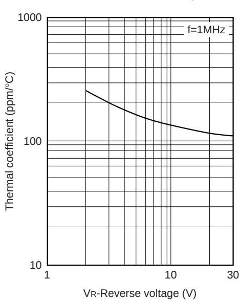
Thermal coefficient of diode capacitance
