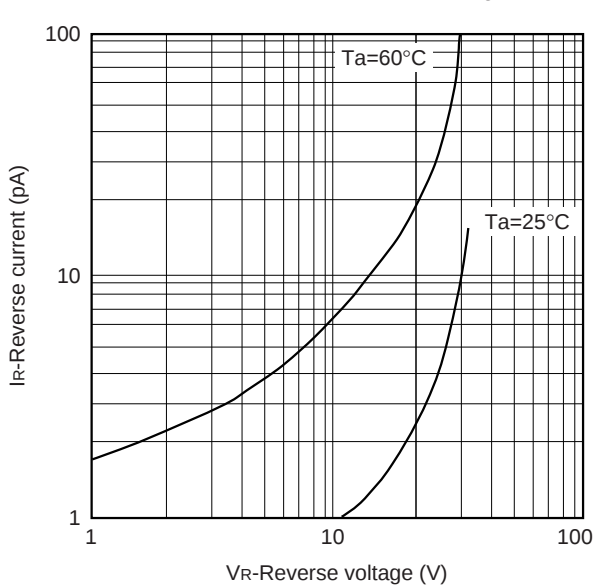
Reverse current vs. Reverse voltage
