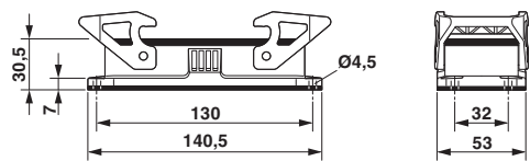
Dimensional drawing
