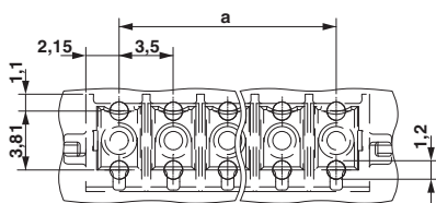
Drilling diagram
