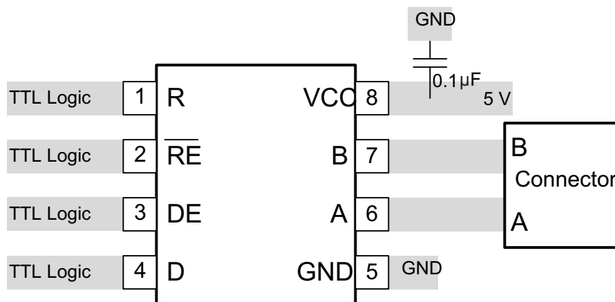
Layout Example
