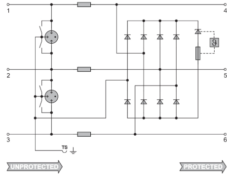
Circuit diagram
