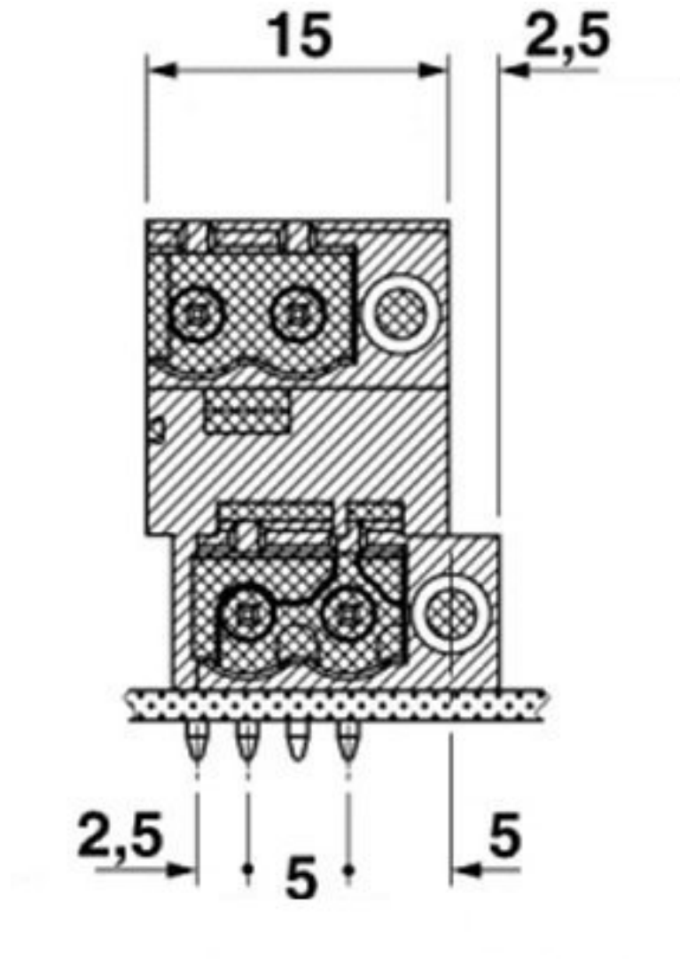
Dimensional drawing
