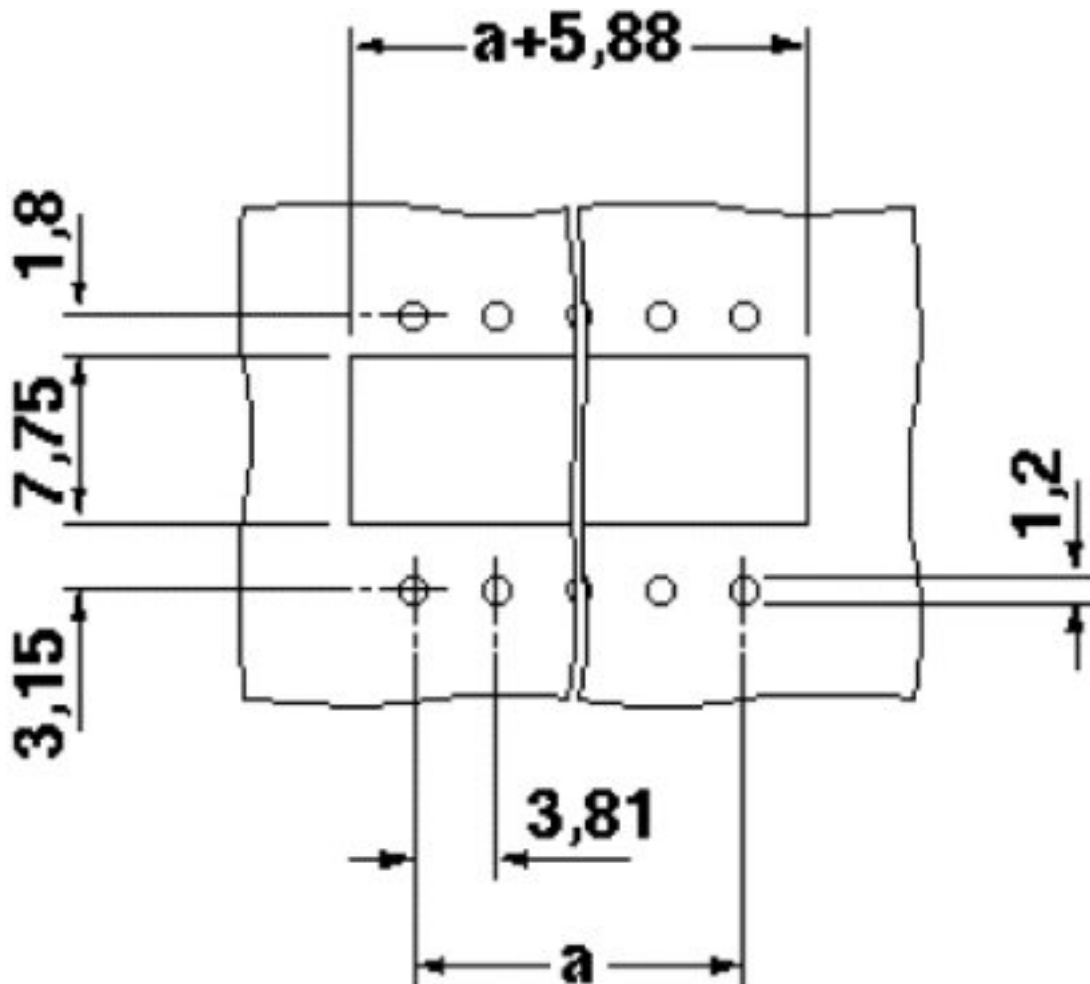
Drilling diagram
