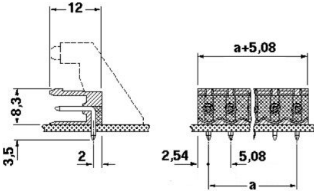
Dimensioned drawing
