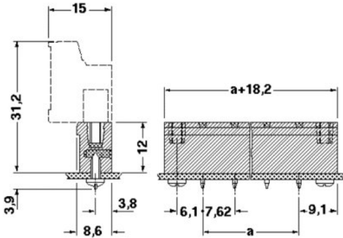
Dimensioned drawing
