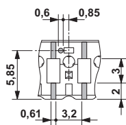
Dimensioned drawing
