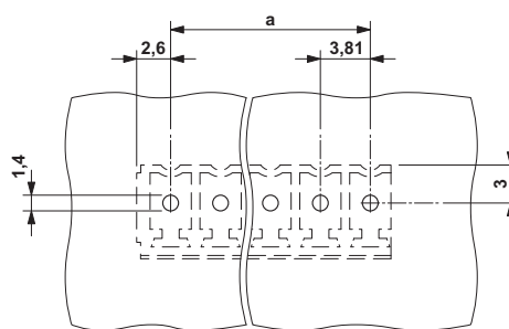
Drilling diagram
