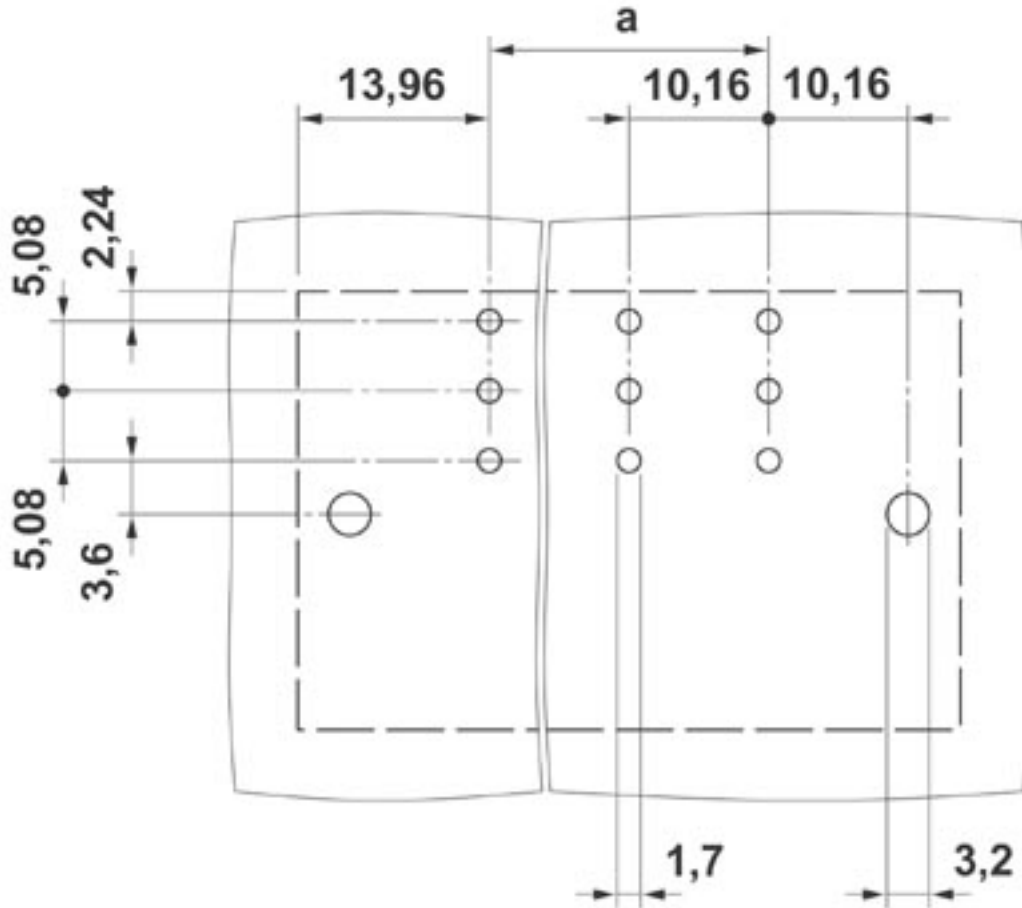
Drilling diagram
