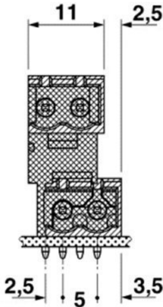
Dimensioned drawing
