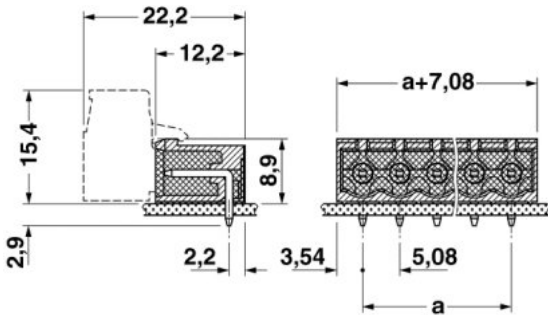
Dimensioned drawing
