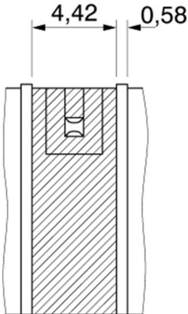
Dimensioned drawing
