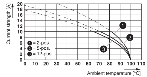
Type: MSTB 2,5/...-ST-5,08 with MDSTBA 2,5/...-G-5,08
