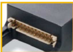
Back Detail 24 Position, 2.0 mm AMPMODU Connector
