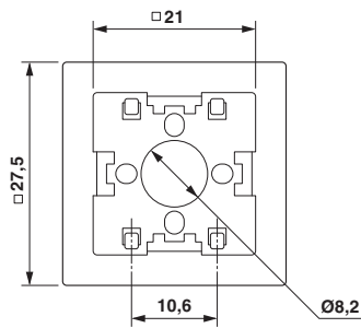
Dimensional drawing
