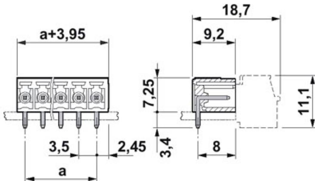
Dimensioned drawing
