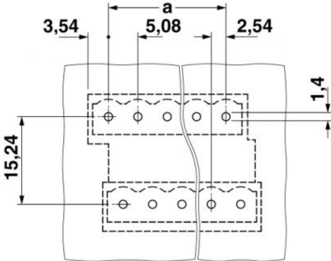
Dimensional drawing
