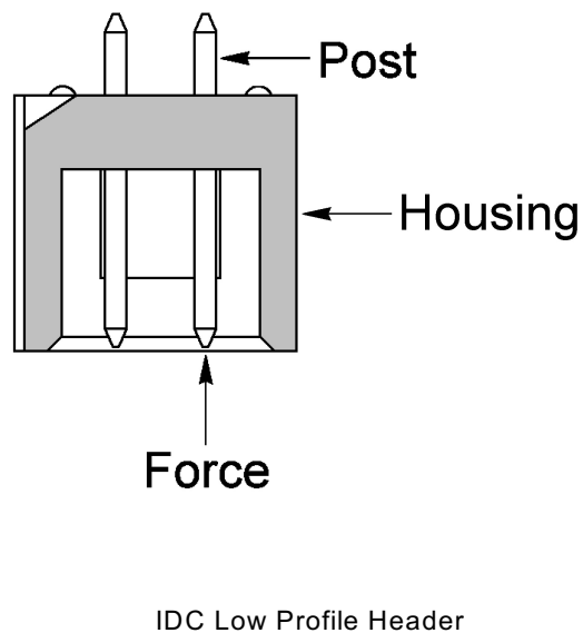
Figure 3 Contact Retention
