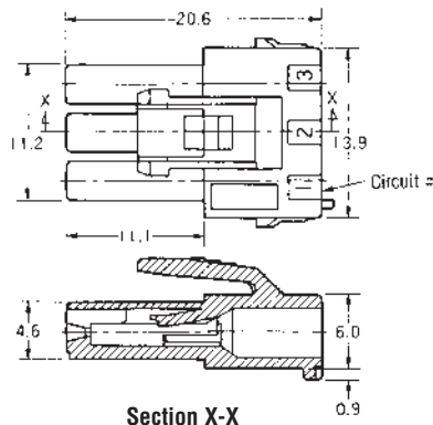
Section X-X
