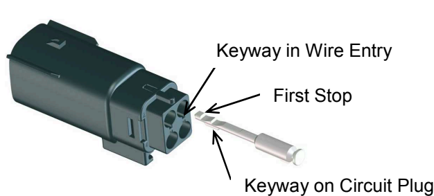
Figure 3: Circuit Plug Orientation
