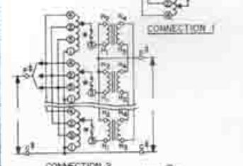
CONNECTION 2
