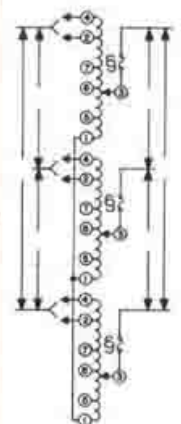
CONNECTION 2
