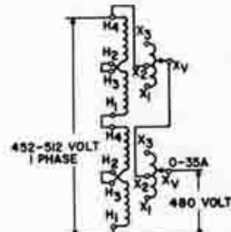
LINE CORRECTOR
