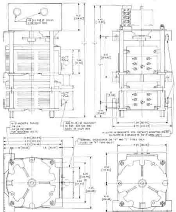
MOTOR DRIVEN
