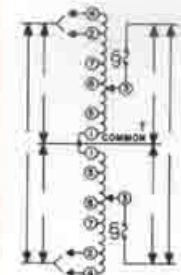
CONNECTION 1
