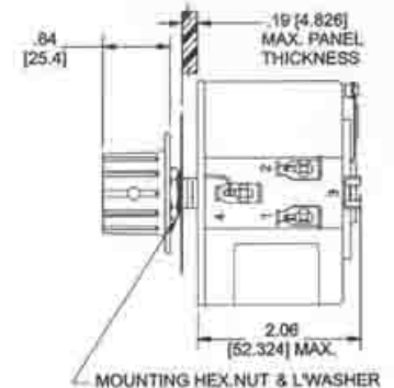
DETAIL OF SHAFT AND BUSHING
