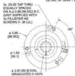
DETAIL OF SHAFT & BUSHING
