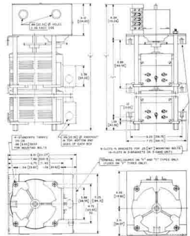
MOTOR DRIVEN
