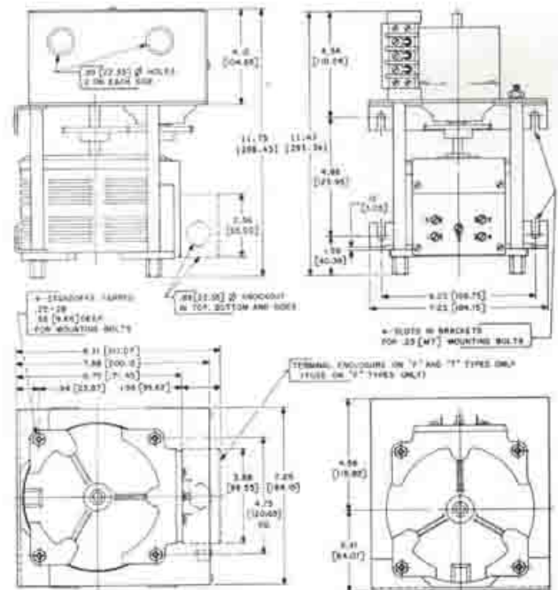
MOTOR DRIVEN
