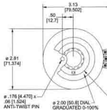
TYPE 12C
