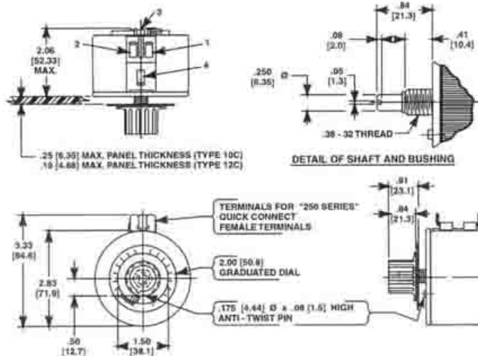
TYPE 10C
