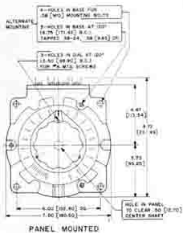
PANEL MOUNTED
