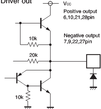
Regulator (base connection)
