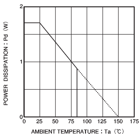
Fig.5 Thermal derating curve (unmounted)
