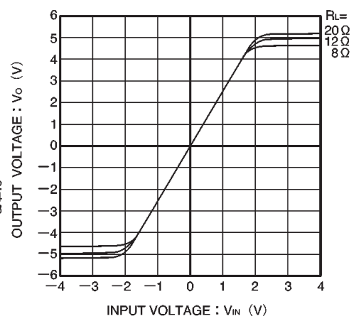
Fig.7 Driver I / O characteristics (during load regulation)
