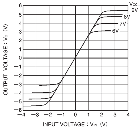
Fig.8 Driver I / O characteristics (power supply regulation)
