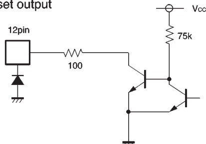
Reset output
