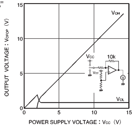
Fig.9 Op-amp high / low level output voltage
