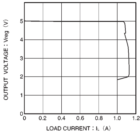
Fig.11 Load current vs. regulator voltage
