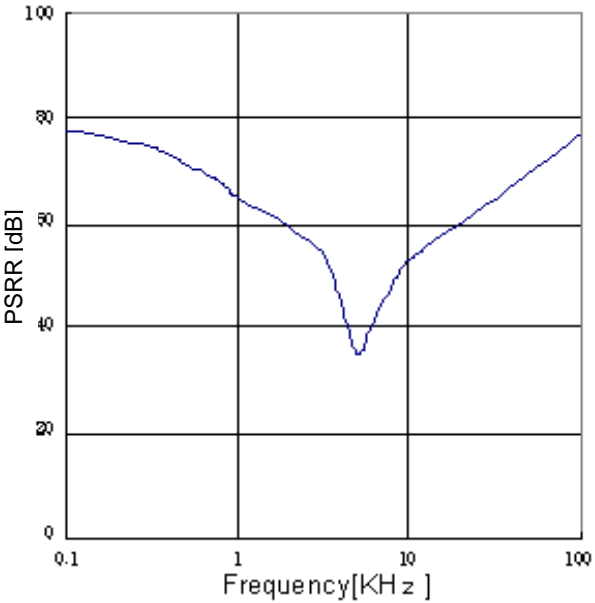
Figure 32. PSRR ( I_o=0\text{mA} )
