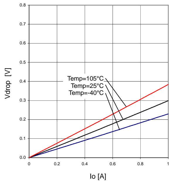
Figure 38. Minimum dropout Voltage 5 ( V_{CC}=12.0V )
