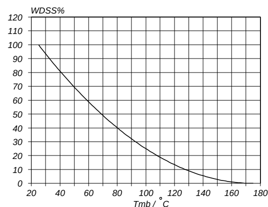
Fig.16. Normalised avalanche energy rating. W_{DS\%} = f(T_{mb}) ; conditions: I_D = 75 \text{ A}
