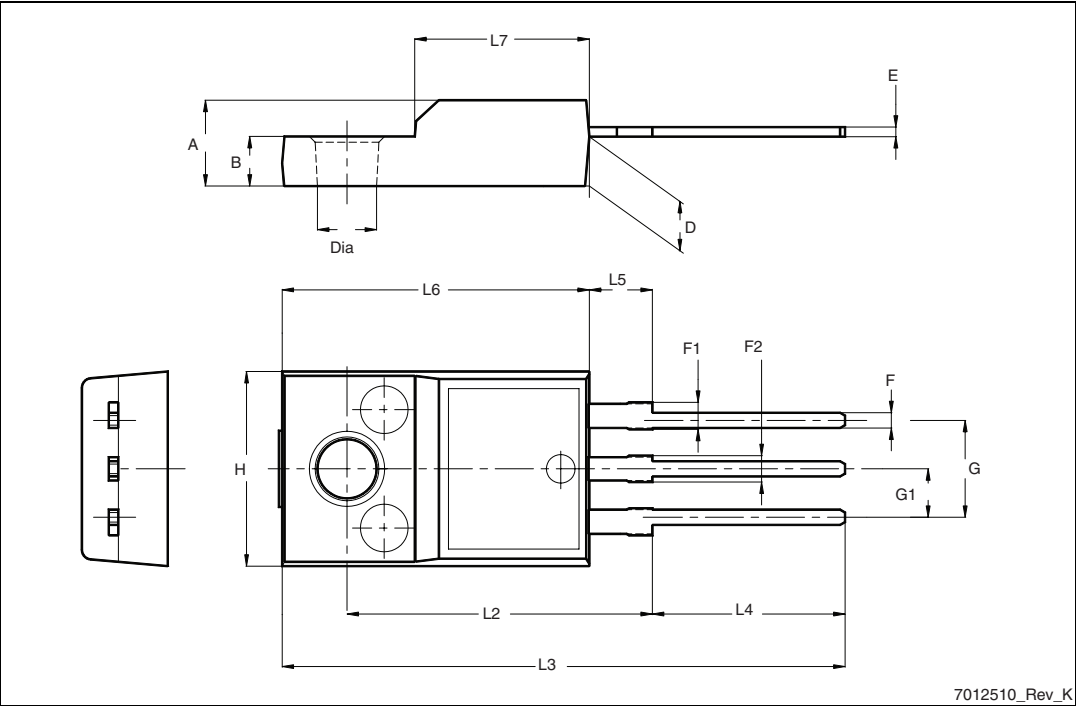
Figure 17. TO-220FP drawing
