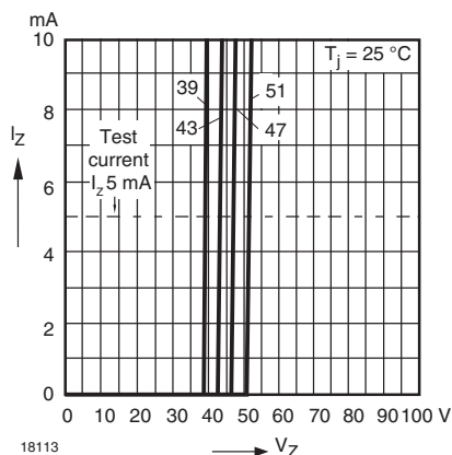
Figure 18. Breakdown Characteristics
