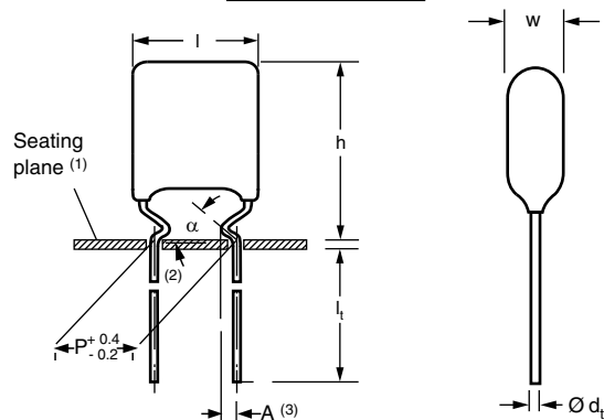
366 Kinked Leads
