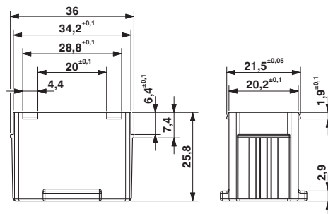
Dimensioned drawing
