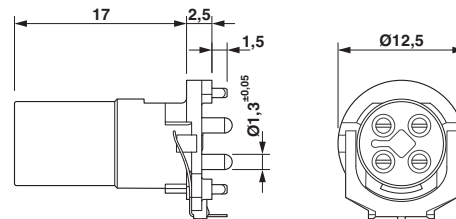
M12 female connector contact carrier
