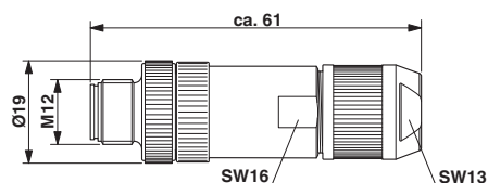
Dimensioned drawing
