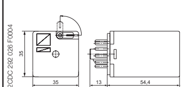
CR-U with 3 c/o contacts
