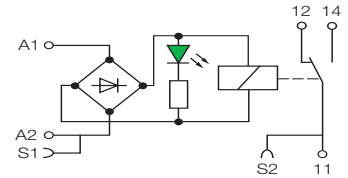
RB/RBR 121 A - 24 V AC/DC
