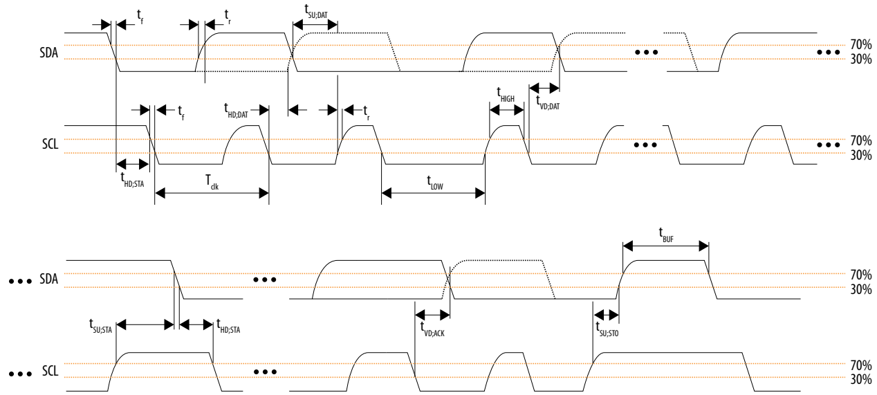
Figure 17: I 2 C Timing Diagram
