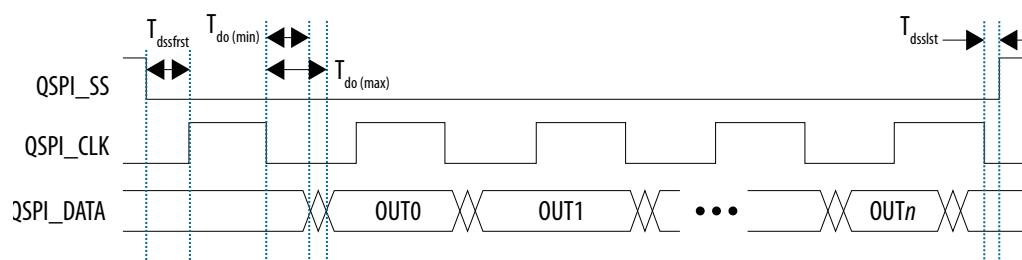
Figure 6: Quad SPI Flash Serial Output Timing Diagram
