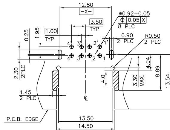
RECOMMEND P.C.B LAYOUT (THICKNESS 1.4~1.6mm) (COMPONENT SIDE) TOLERANCE±0.05mm
