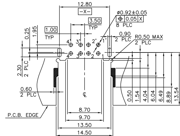
RECOMMEND P.C.B LAYOUT (THICKNESS 1.4~1.6mm) (COMPONENT SIDE) TOLERANCE±0.05mm
