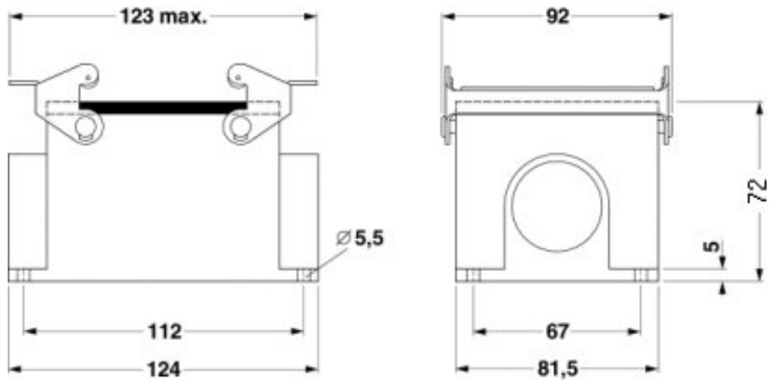
Dimensioned drawing
