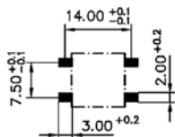
Gullwing lead
