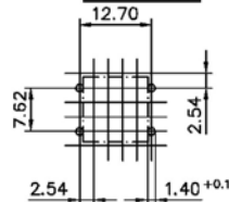
PCB lead
