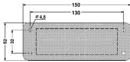
Adapter plate
