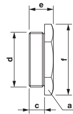
Dimensioned drawing
