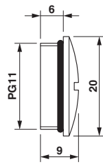
Dimensioned drawing
