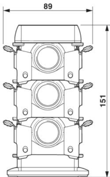
Dimensional drawing
