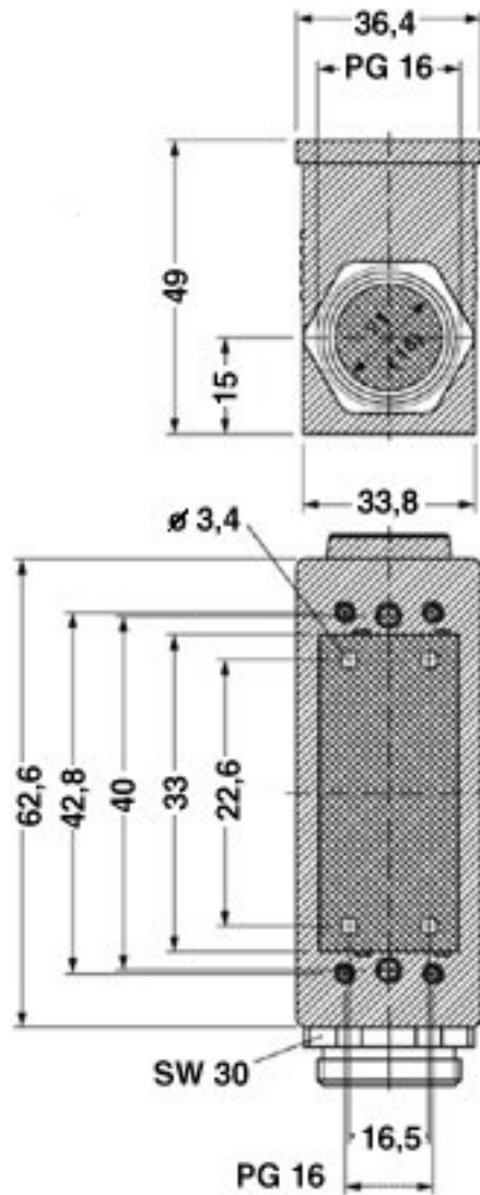
Dimensional drawing
