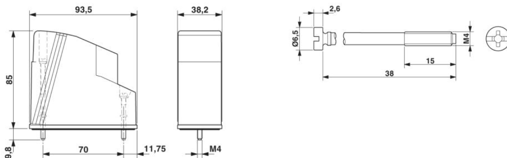
Dimensioned drawing
