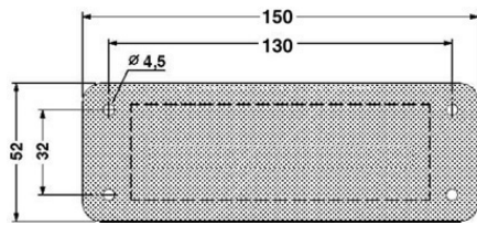
Adapter plate
