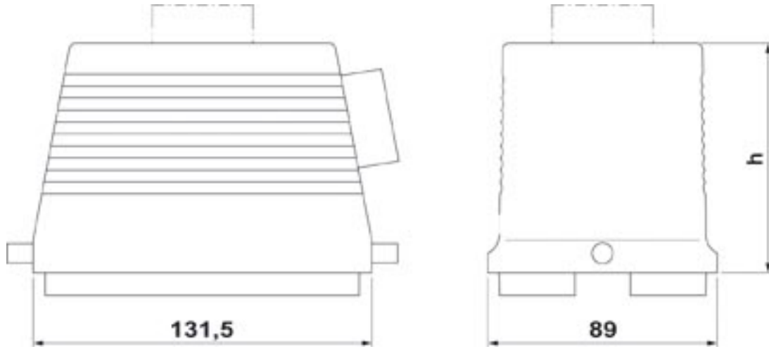
Dimensioned drawing
