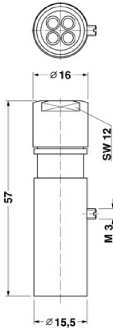
Dimensioned drawing
